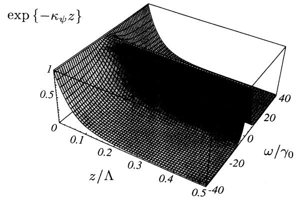
FIG. 7. Damping of initial above-shot-noise fluctuations for symmetric situation and \Omega^2 = 5\gamma\gamma_0 as a function of propagation distance z and Fourier frequency \omega .
