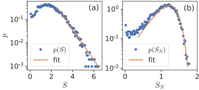
FIG. 7. Distribution of saturation values for the free fermion model with off-diagonal disorder, Eq. (A1), for L = 1024 using 20 000 disorder realizations: (a) von Neumann entropy and (b) number entropy. Symbols represent numerical data, the line in (a) is an exponential fit p(S) \sim e^{-(3/2)S} , and the line in (b) is the corresponding fit for S_N using the relation (4), p(S_N) \sim \exp[4(S_N - \gamma)] \exp\{-\frac{3}{2} \exp[4(S_N - \gamma)]\} with \gamma = \ln 3.75 . Here the constants are fit parameters.
