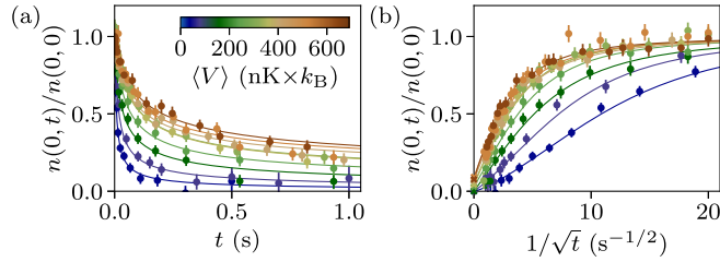
FIG. 11. Determining the localized fraction f_{\text{loc}} . (a) Relative peak density n(t)/n(0,0) (circles) over expansion time t . Lines are fits with the anomalous-diffusion model Eq. (E2) where f_{\text{loc}} , the value for t \rightarrow \infty is the only free parameter. Errors are calculated from error propagation. (b) Plotting n(t)/n(0,0) over the inverse square root of time visualizes f_{\text{loc}} as the density-axis intercept (crosses).
